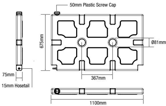
IWT003 - 40L VERTICAL TANK
