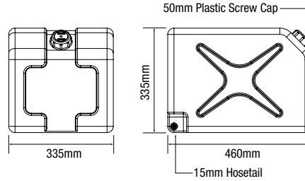
IWT002 - 40L JERRY CAN
