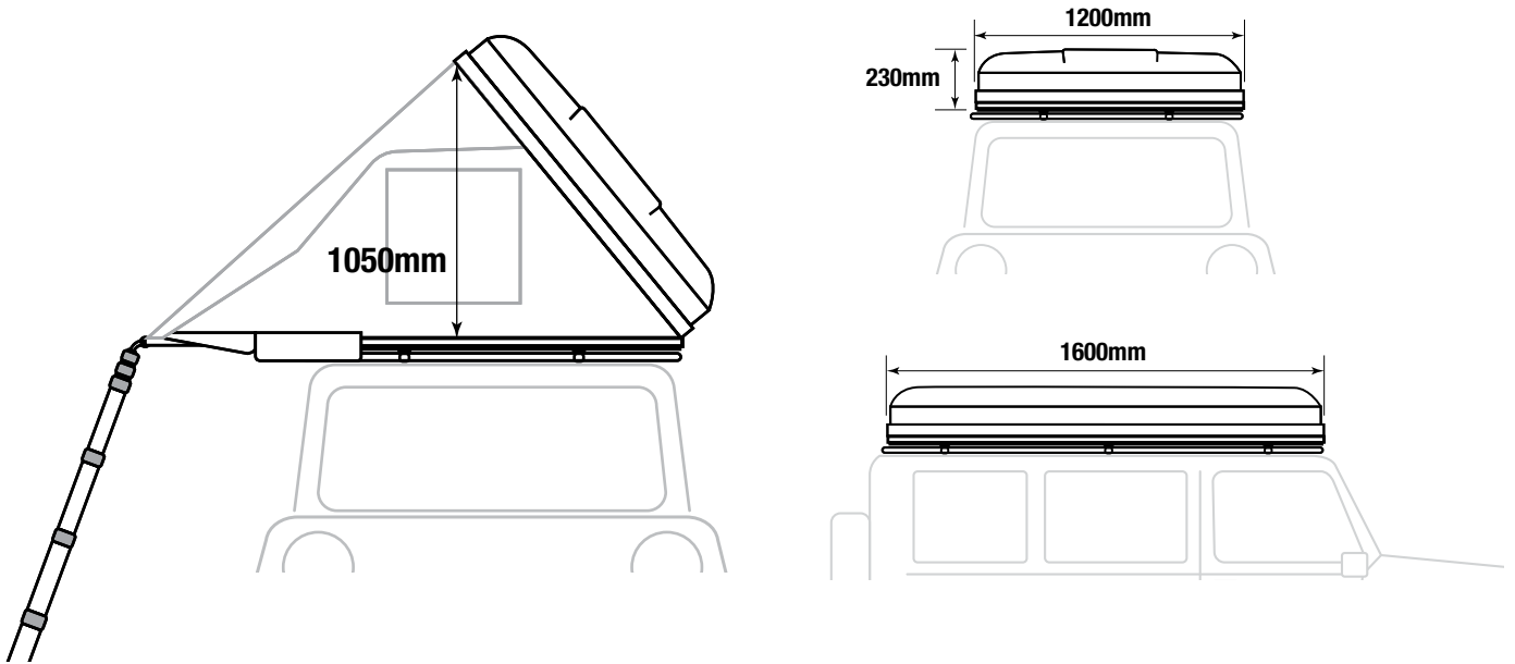
NOMAD 1300 ABS ROOFTOP TENT - (WEIGHT 69KG)
