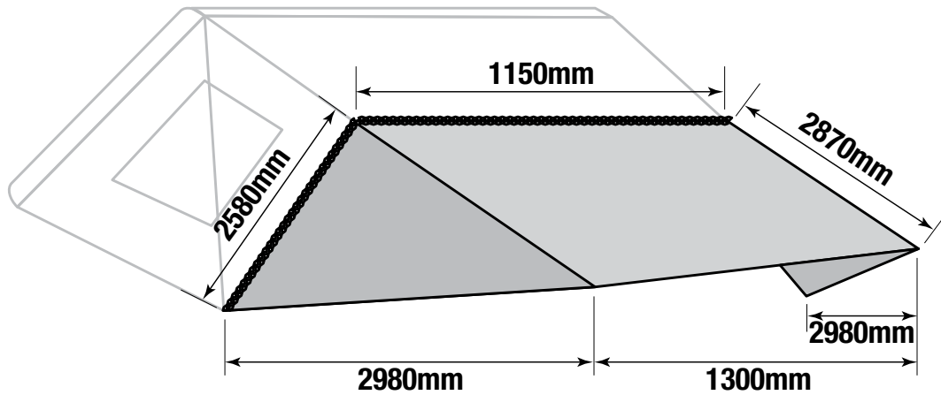
NOMAD 1300 ROOFTOP TENT AWNING - (WEIGHT 3KG)
