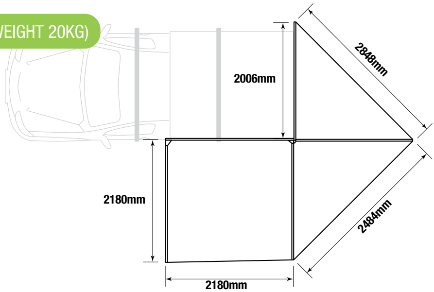
DELTAWING 270 XTR-71 - (WEIGHT 20KG)
