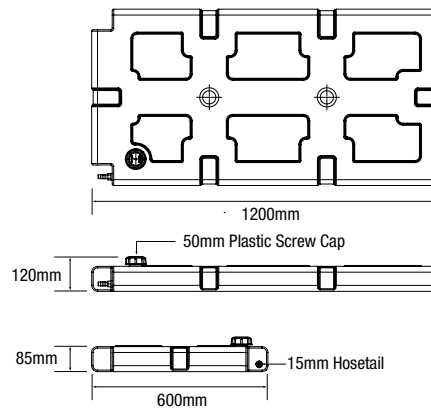
IWT004 - 50L ROOF RACK TANK
