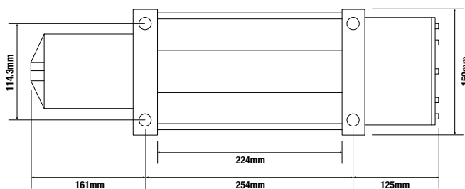
BOLTING PATTERN
