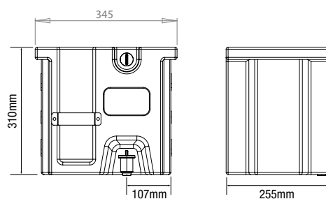
IWT008 - 15L UNDER TRAY HAND WASH TANK
