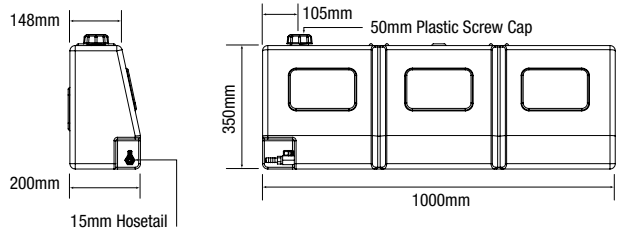
IWT006 - 50L TAPERED TANK
