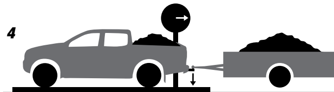
4 Vehicle with trailer connected minus total weight of vehicle = Ball weight Ensure total weight of vehicle including ball weight does not exceed manufacturers GVM
