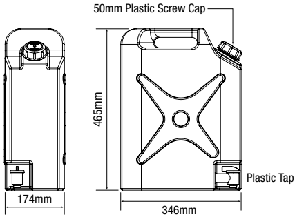
IWT003 - 40L VERTICAL TANK
