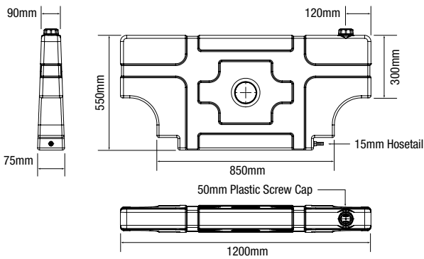
IWT005 - 50L WHEEL ARCH TANK
